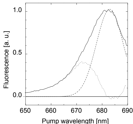
FIGURE 7 Deconvolution of the fluorescence spectrum (solid line) between 670 and 690 nm into a Gaussian subband (dashed line) at 683 \text{ nm} with a FWHM of 260 \text{ cm}^{-1} (cf. Fig. 6) and additional fluorescence band(s) with a maximum \sim 672 \text{ nm} (dotted line).
